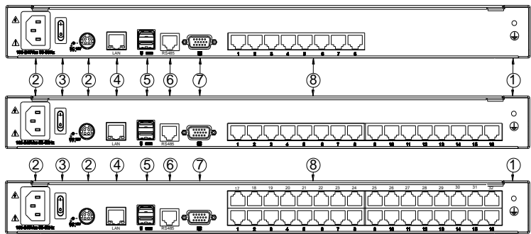
Figure 1.3 Rear view
